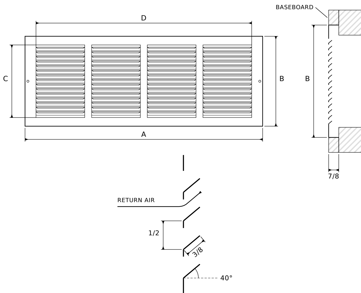
LOUVER DETAIL
