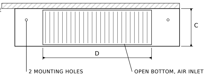
BOTTOM VIEW
